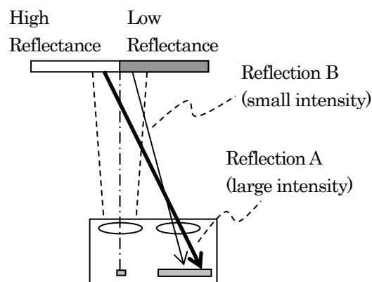
Fig.07 Reflective object with boundary line
