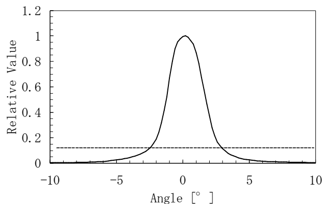
Fig.10 Example of Directional Angle of Emitting Beam
