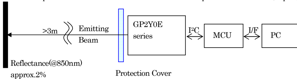
Fig.27 Example of measurement environmental of cover compensation coefficient
