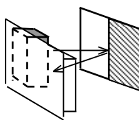
Fig.08 Recommended measurement of reflective object with boundary line
